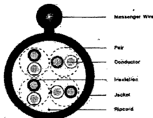
US-9045 : OUTDOOR CAT 5E (DOUBLE JACKET) 2.6.3
